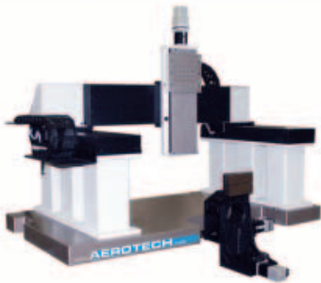
5-axis precision laser cutting & welding station
