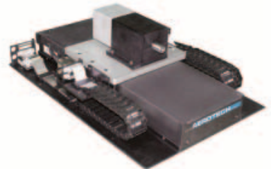
High throughput cylindrical laser cutting system
