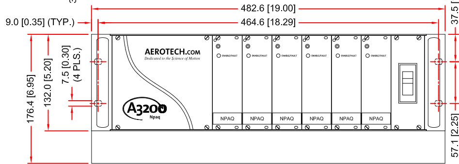
NPAQ WITH FAN TRAY OPTION
