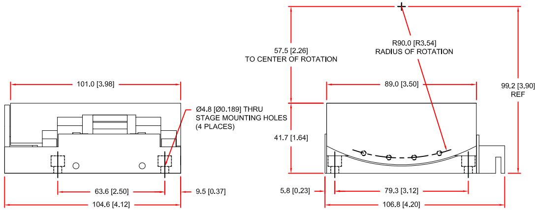
DIMENSIONS - MILLIMETERS [INCHES]
