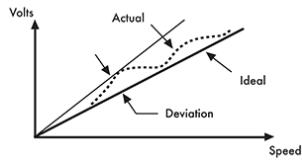
Tachometer
