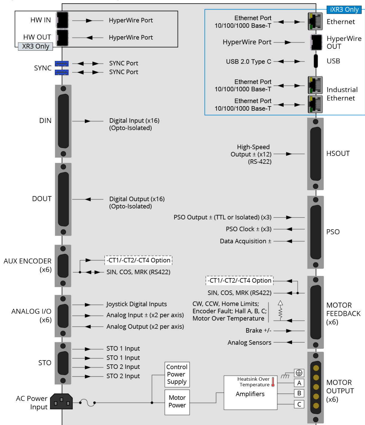
Figure 1-3: Functional Diagram
