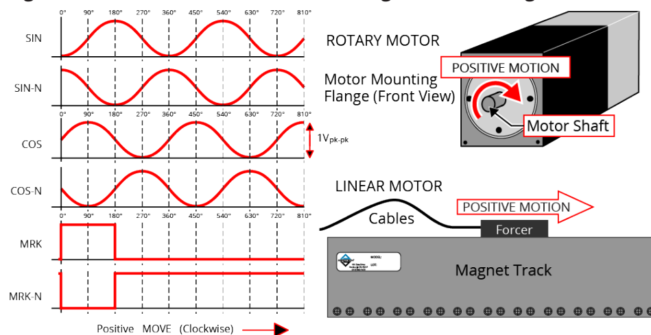
Figure 2-41: Sine Wave Encoder Phasing Reference Diagram
