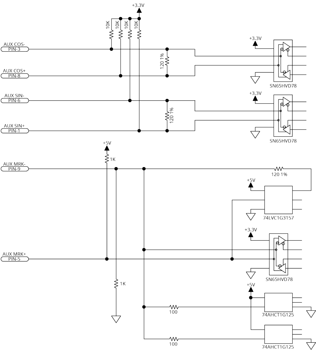
Figure 2-39: Square Wave Encoder Interface (Aux Encoder Connector)
