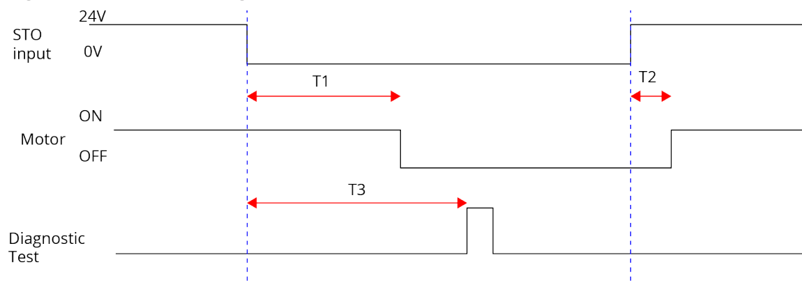
Figure 2-48: STO Timing
