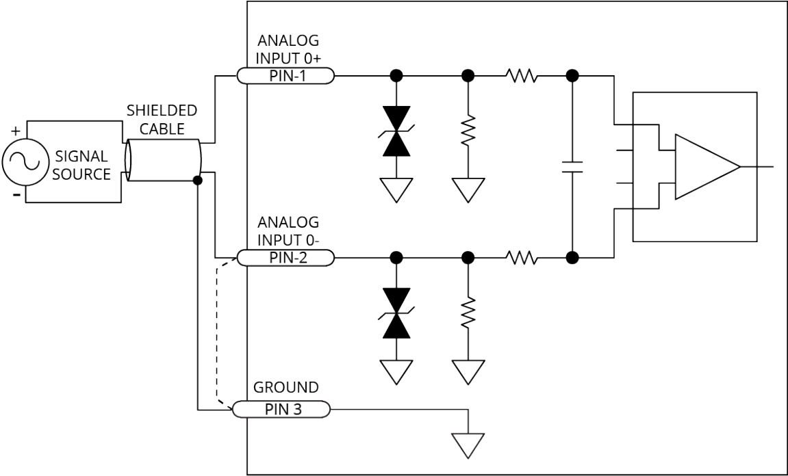
Figure 2-44: Analog Inputs Schematic
