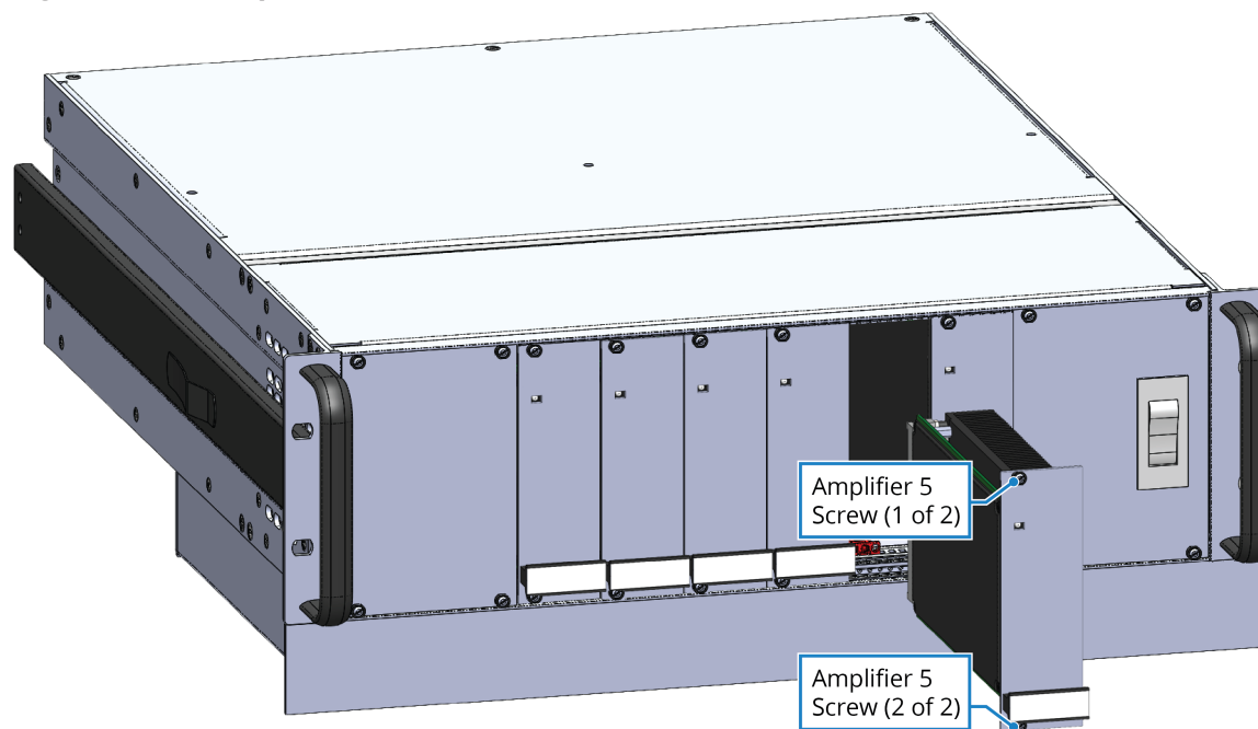
Figure 3-2: Amplifier Removal
