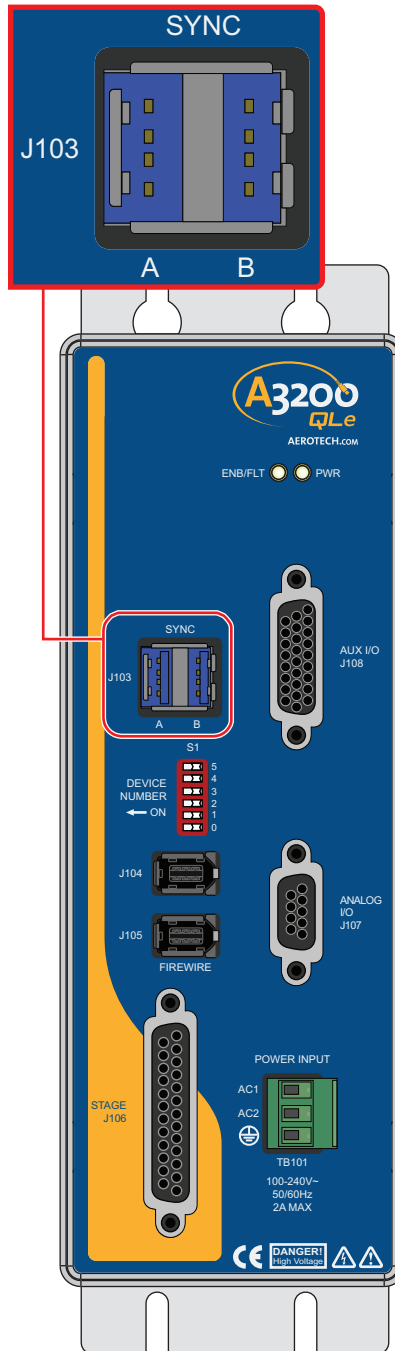
Figure 2-11: Sync Interface
