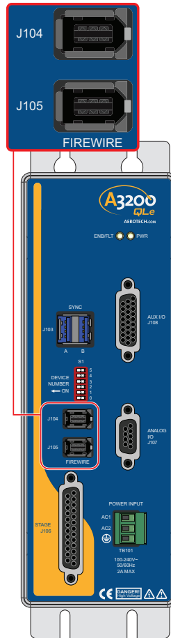
Figure 2-10: FireWire Interface
