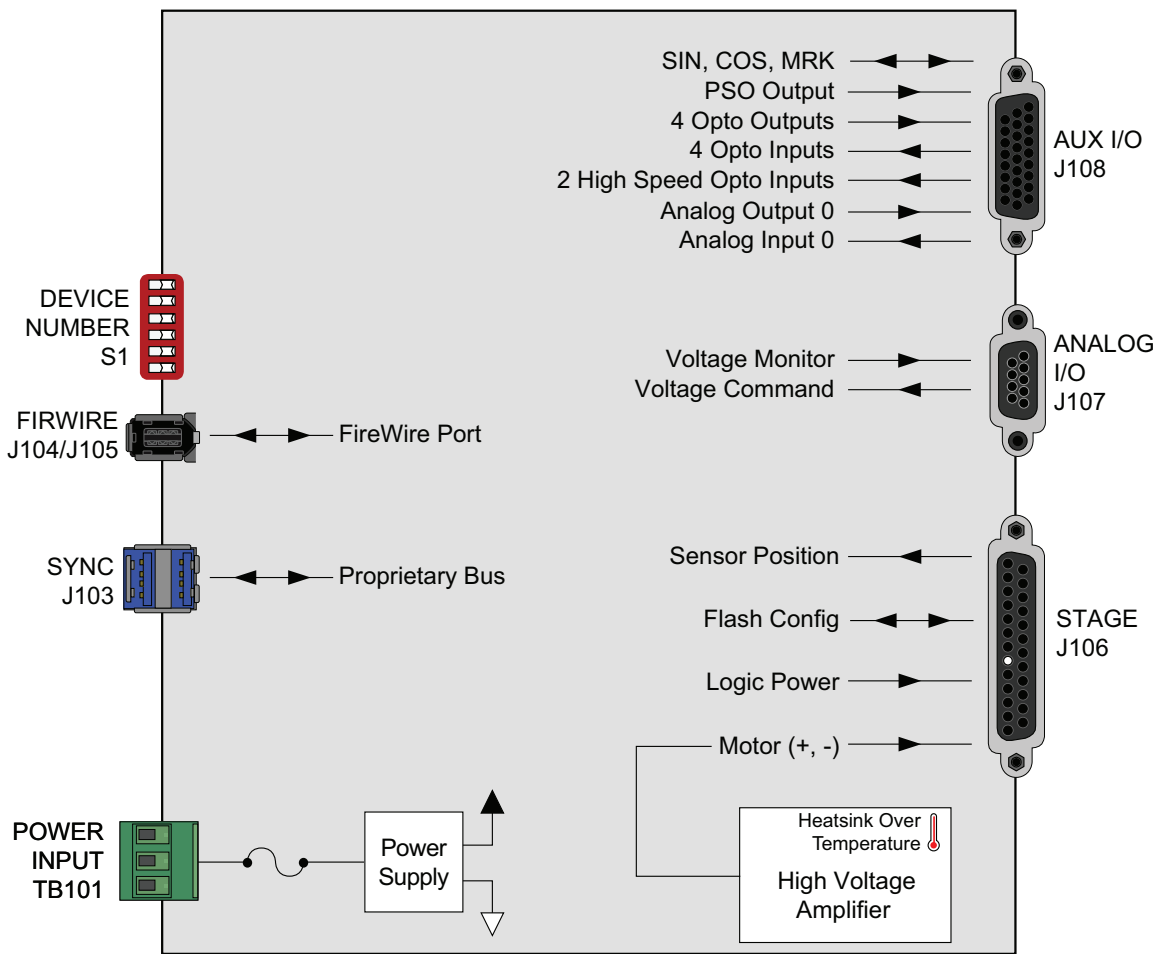
Figure 1-1: Functional Diagram
