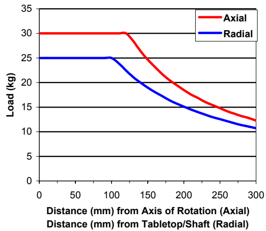
Axial and Radial Cantilevered Load Capability (ADRT150-115)
