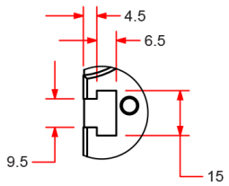
DETAIL A T-SLOT, TYPICAL 8 PLACES
