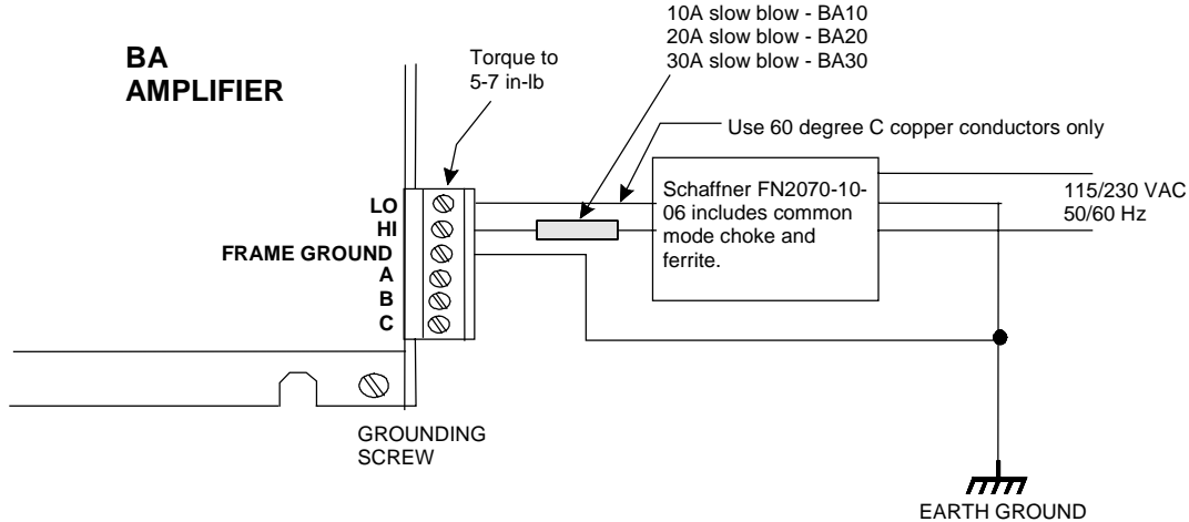
This configuration is especially important if the BA amplifier is operating at DC bus voltages of 160 VDC or 320 VDC (e.g., 115 VAC or 230 VAC input power).
