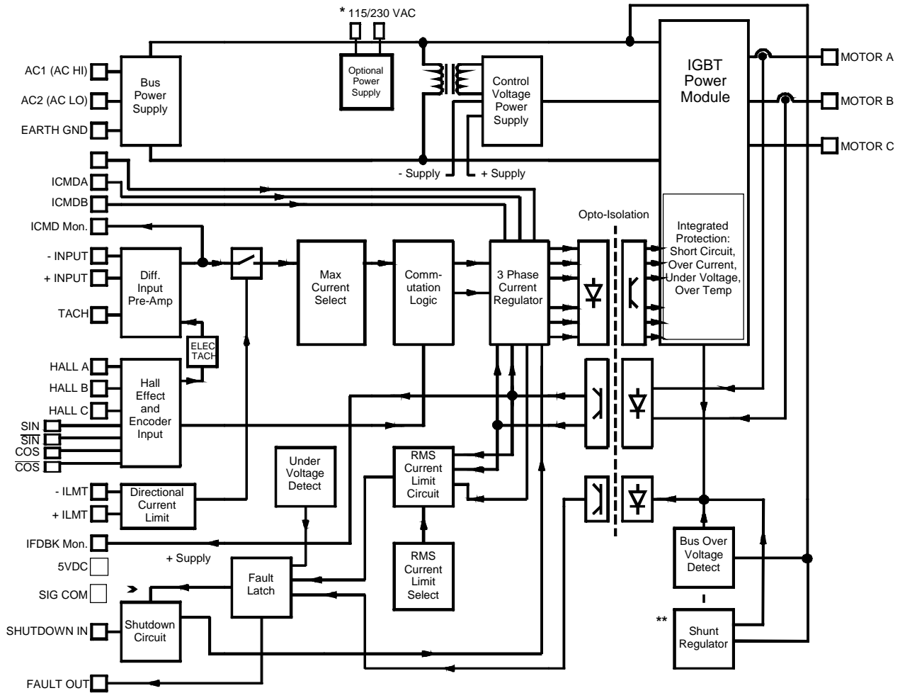
Figure 1-2. Functional Diagram
