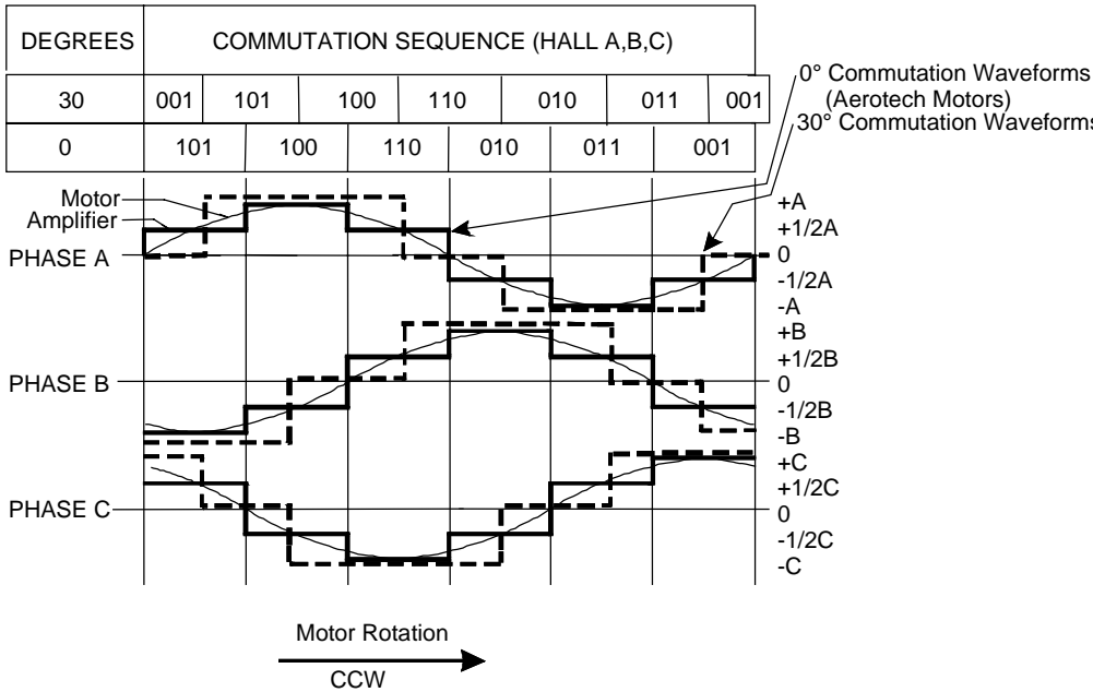
Figure 2-11. Motor Phasing
