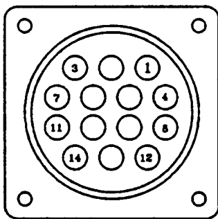
14 Pin Plastic Style * (Standard for U12R and U12S)
