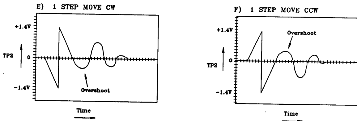
Diagram 4-2: Analog Lock Signal at TP2 for X1,X2 and X4 Resolution (shown for Sine Wave Encoders only)
