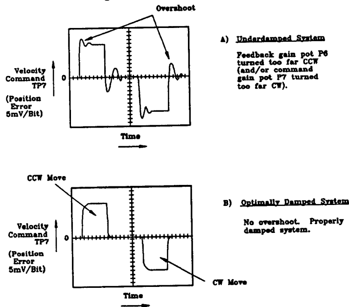
Diagram 4-1: Velocity Command refers to TP7 for Underdamped (A), and Optimally Damped (B), Position Loop Response
