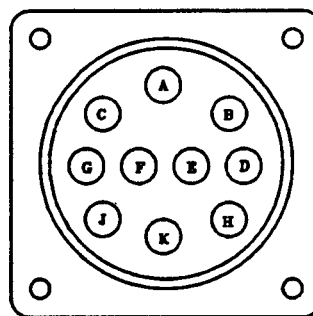
10 Pin Metal Style * (Standard for U12H Chassis Optional for U12R and U12S Chassis)
