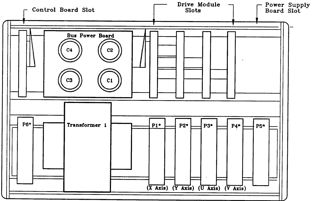
FRONT VIEW
