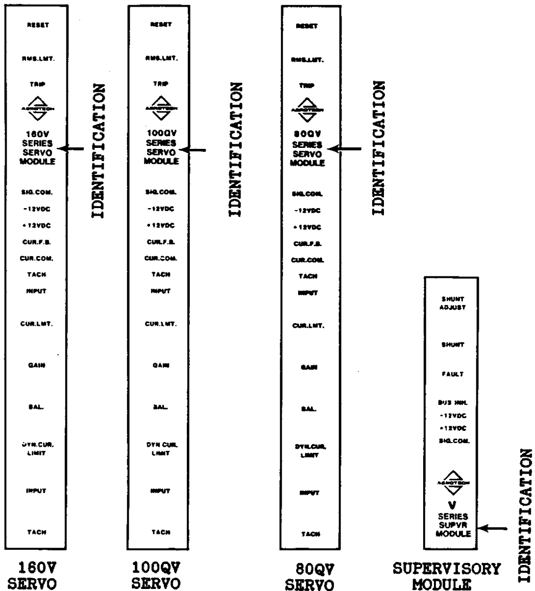
FIGURE 2-2: MODULE IDENTIFICATION LOCATIONS
