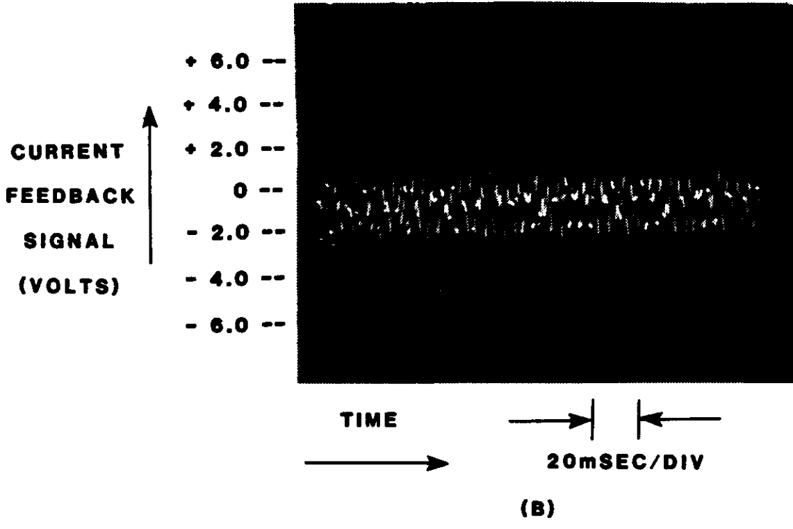
FIGURE 3-10: ADJUSTABLE GAIN POT TO MINIMIZE RIPPLE CURRENT IN MOTOR
