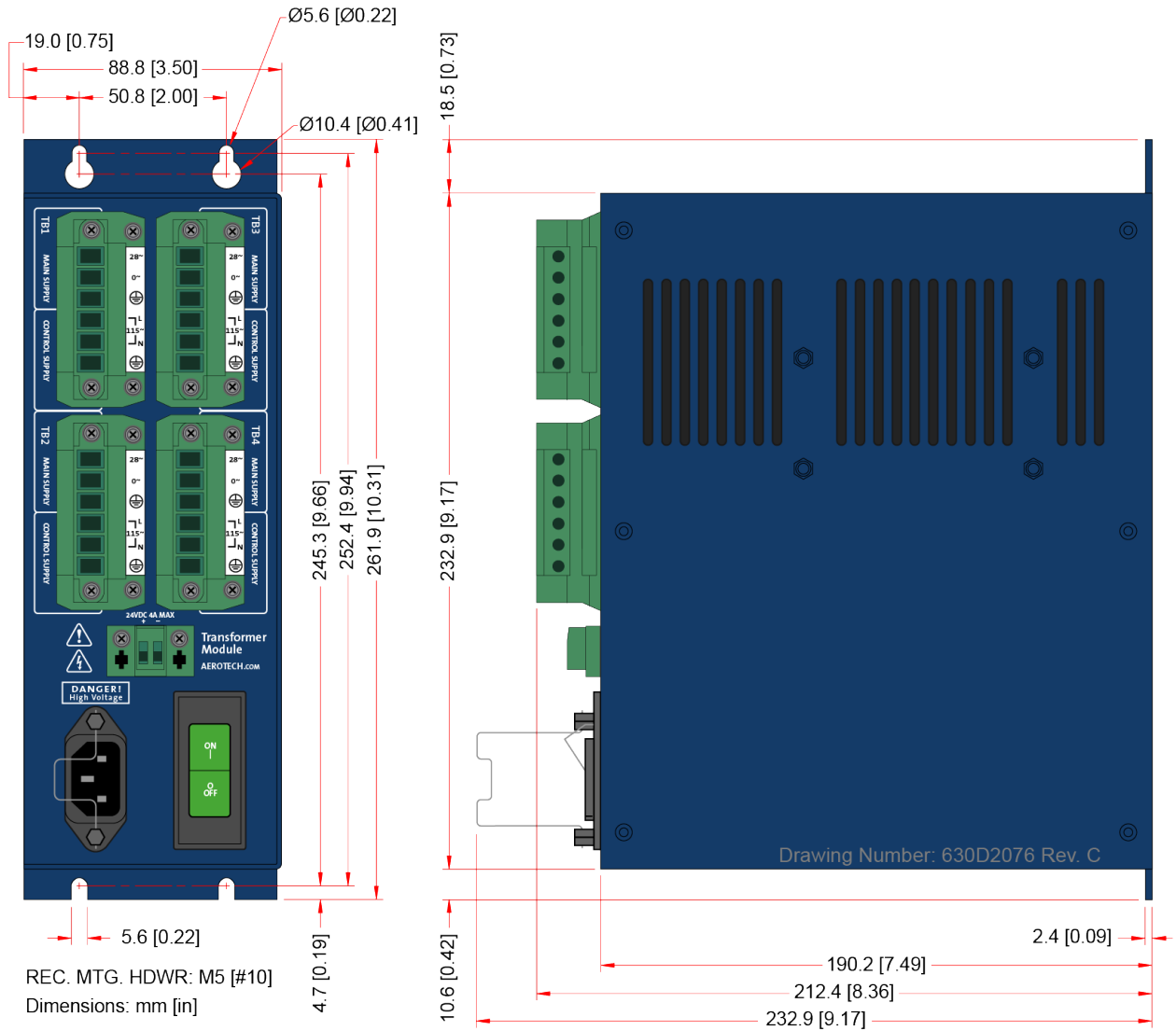
Figure 1-2: TM5 Dimensions
