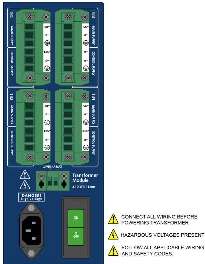
Figure 1-1: TM5 Transformer Module
