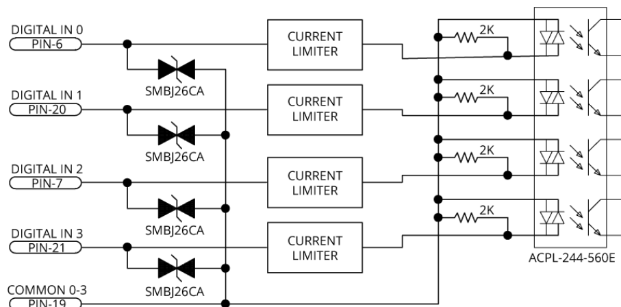
Figure 2-6: Digital Inputs Schematic
