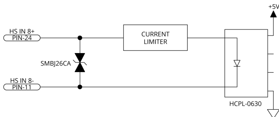
Figure 2-9: High-Speed Input
