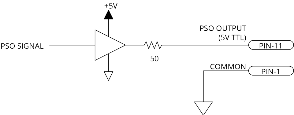
Figure 2-11: PSO TTL Outputs Schematic
