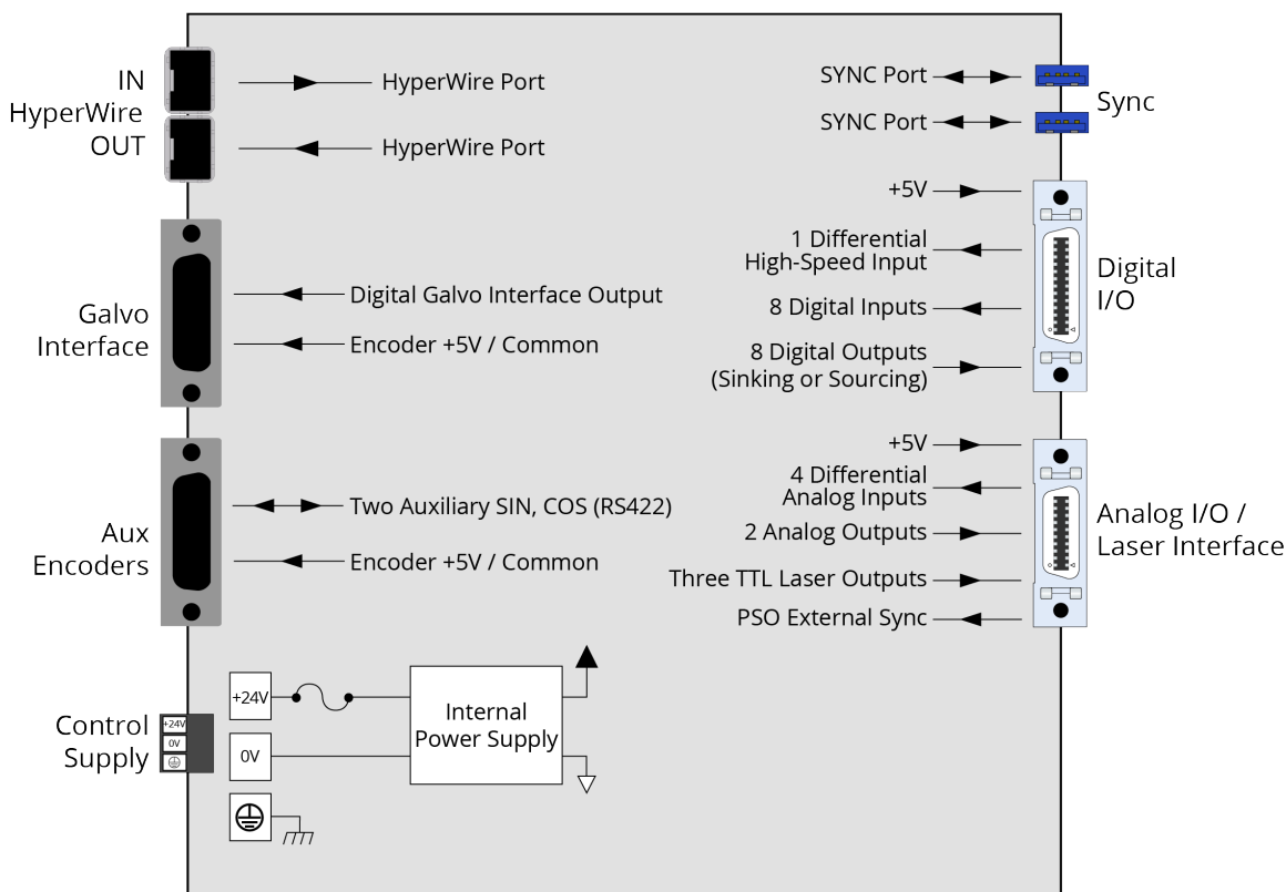
Figure 1-3: Functional Diagram
