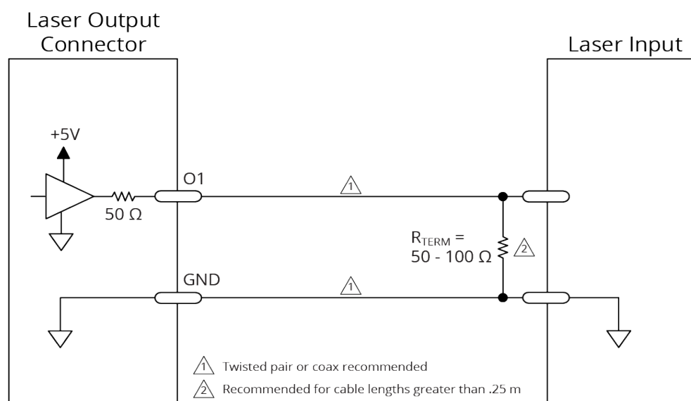
Figure 2-10: TTL Output
