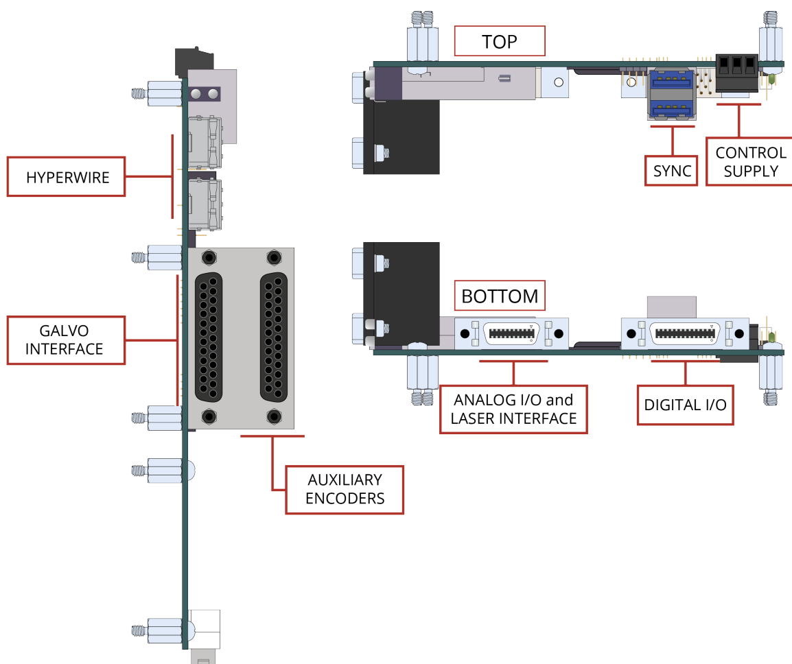
Figure 1-2: GI4-OEM Galvo Scanner Controller
