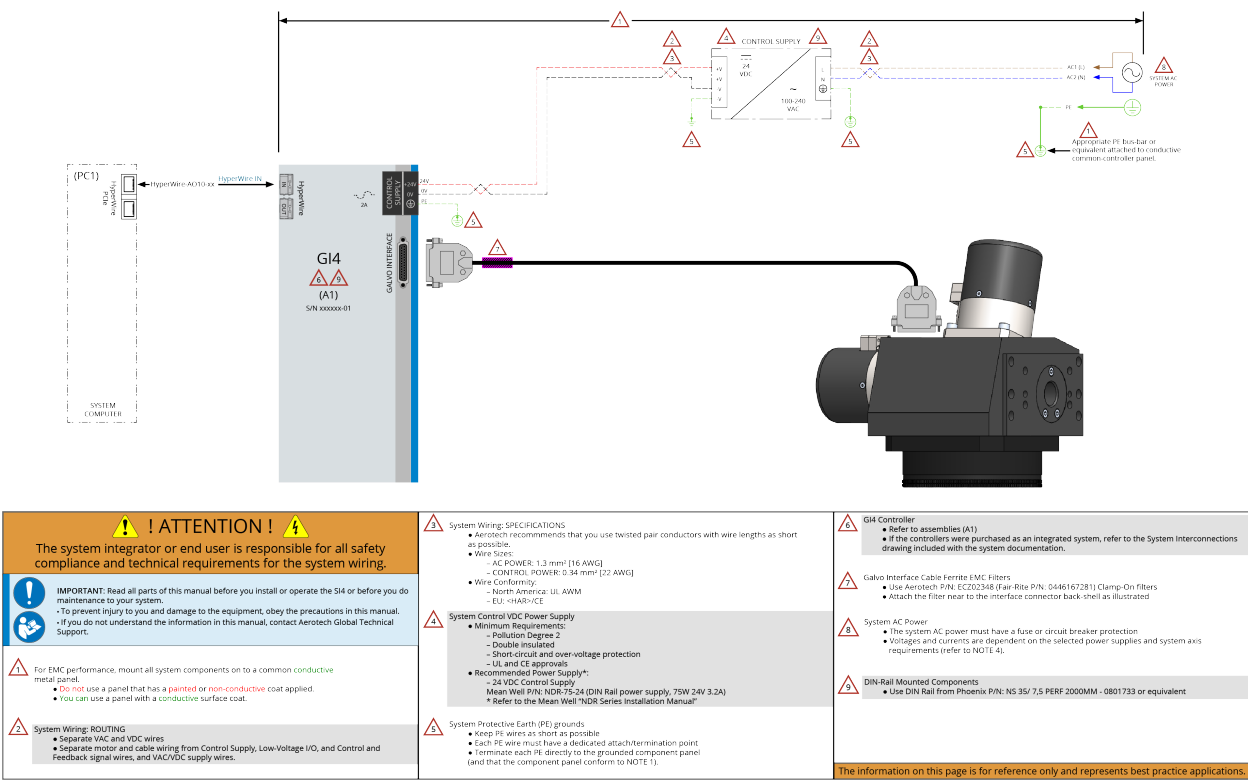
Figure 2-15: System Interconnection Drawing (Best Practice)
