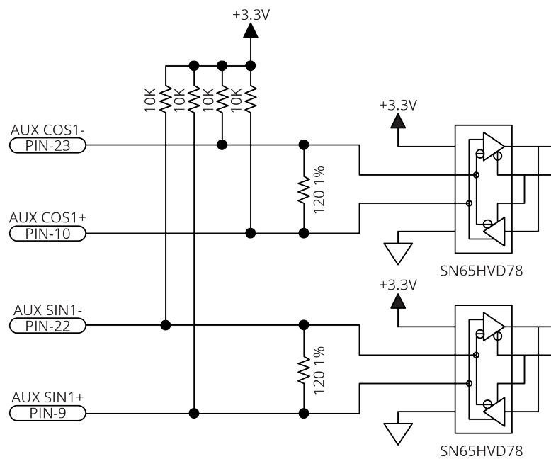
Figure 2-2: Square Wave Encoder Interface
