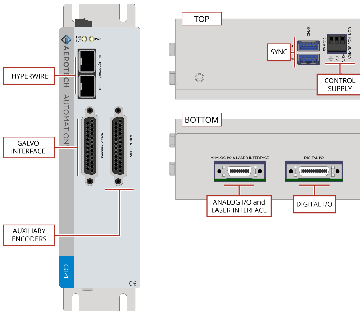
Figure 1-1: GI4 Galvo Scanner Controller
