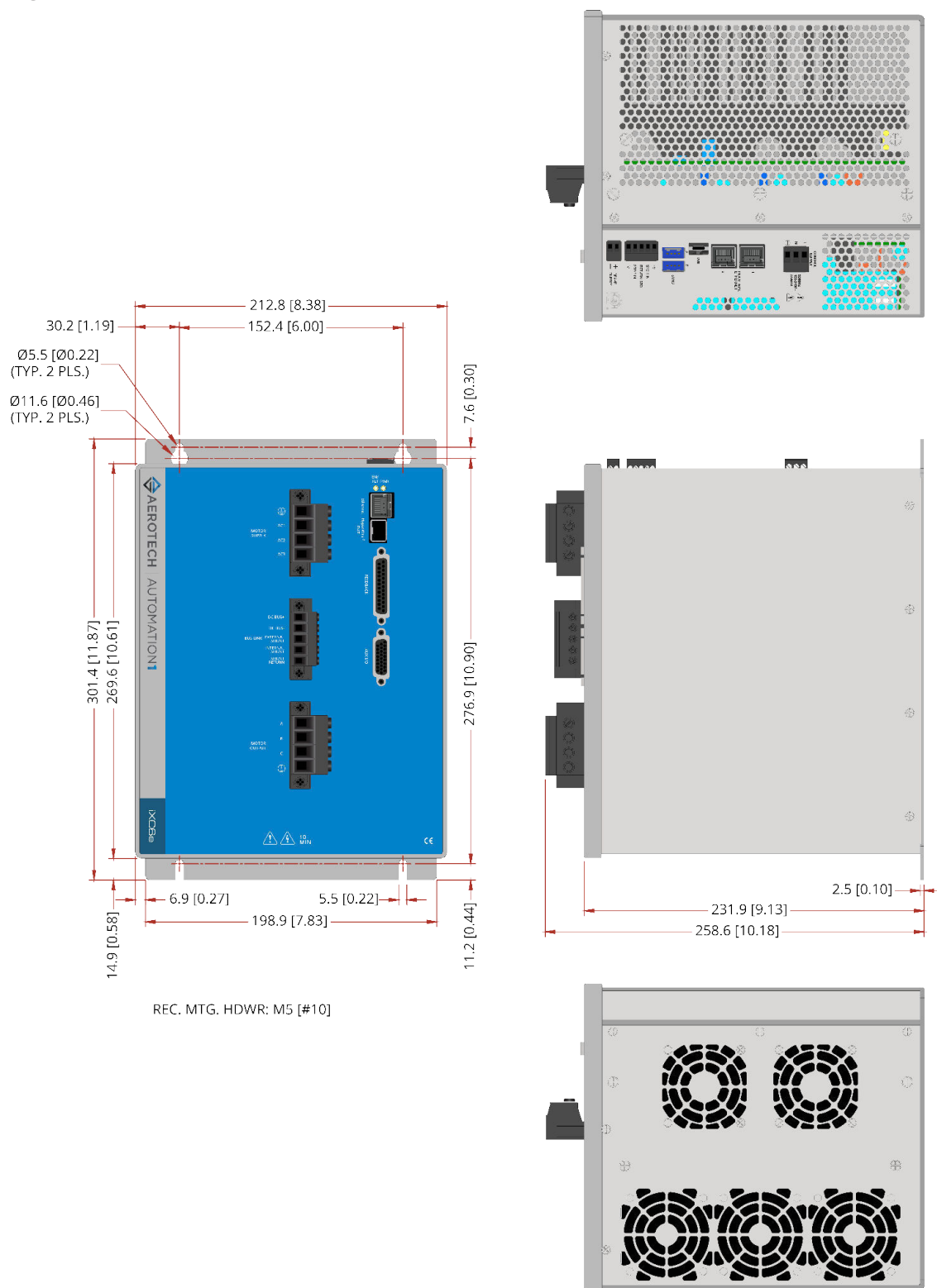
Figure 1-4: Dimensions
