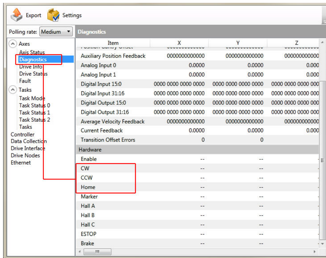
Figure 2-20: End of Travel and Home Limit Input Diagnostic Display
