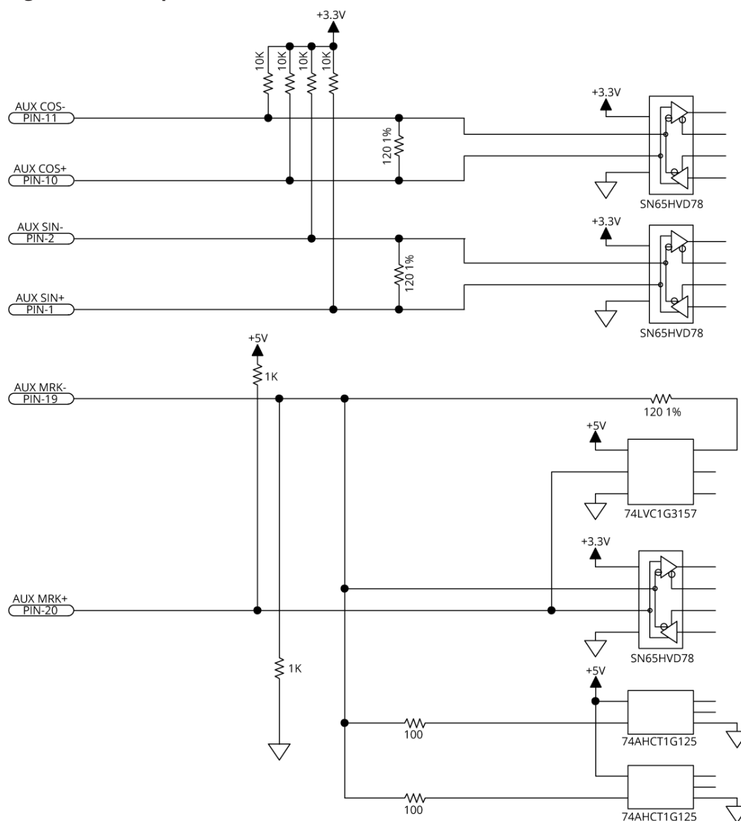
Figure 2-24: Square Wave Encoder Interface (Aux I/O Connector)
