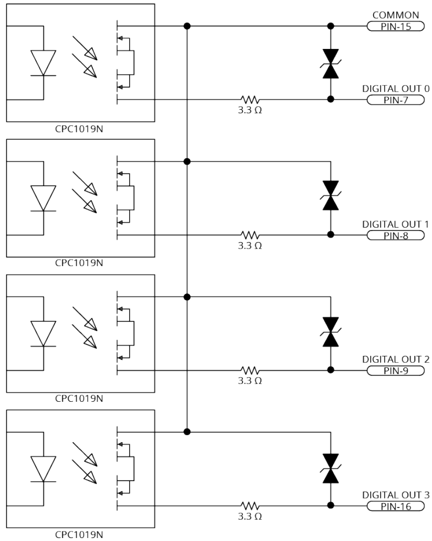
Figure 2-29: Digital Output Schematic (Aux I/O Connector)
