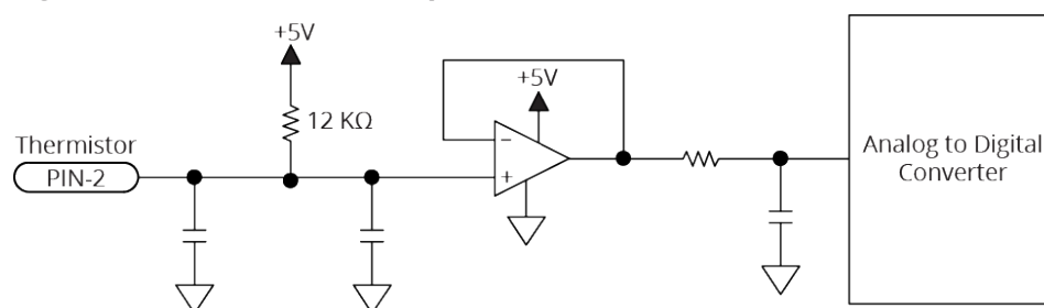
Figure 2-16: Thermistor Input Schematic (Feedback Connector)
