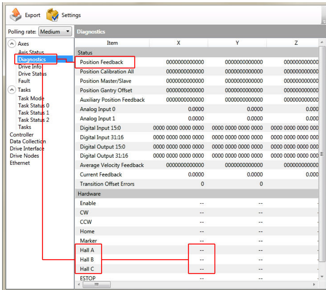
Figure 2-6: Encoder and Hall Signal Diagnostics
