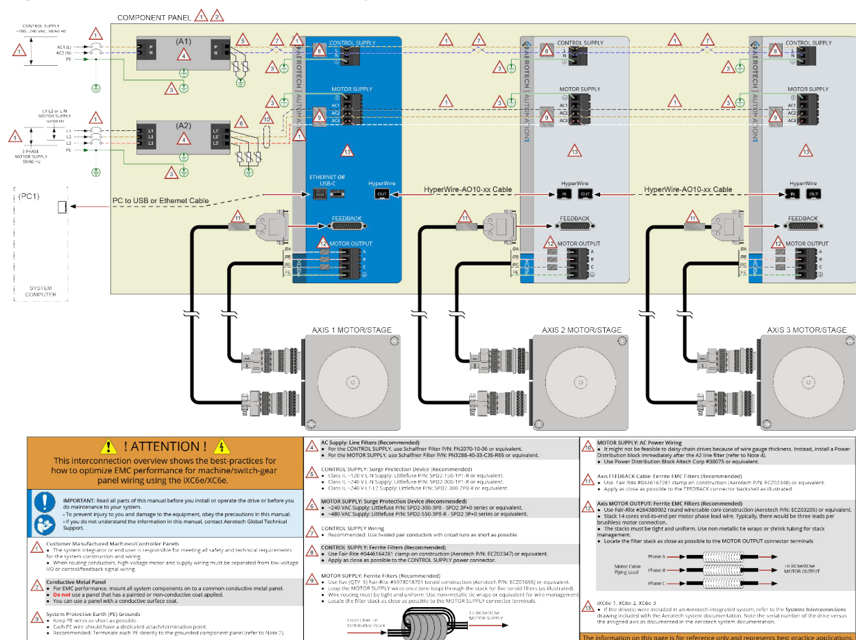
Figure 2-40: Drive-Based Controller System Interconnection (Best Practice)
