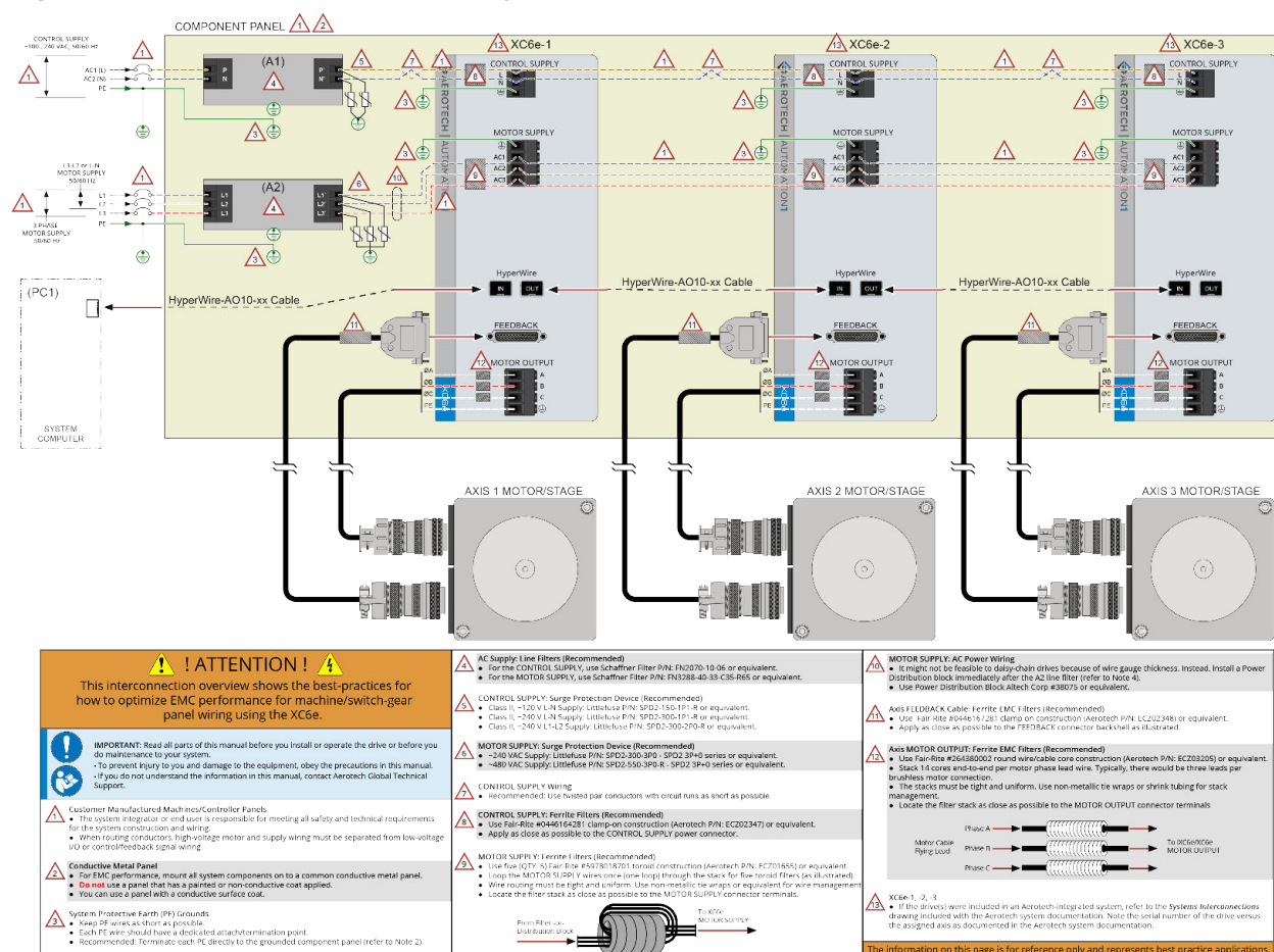
Figure 2-41: PC-Based Controller System Interconnection (Best Practice)
