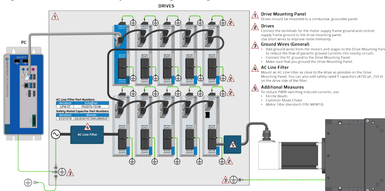
Figure 2-38: Drive-Based System Wiring Drawing (Best Practice)
