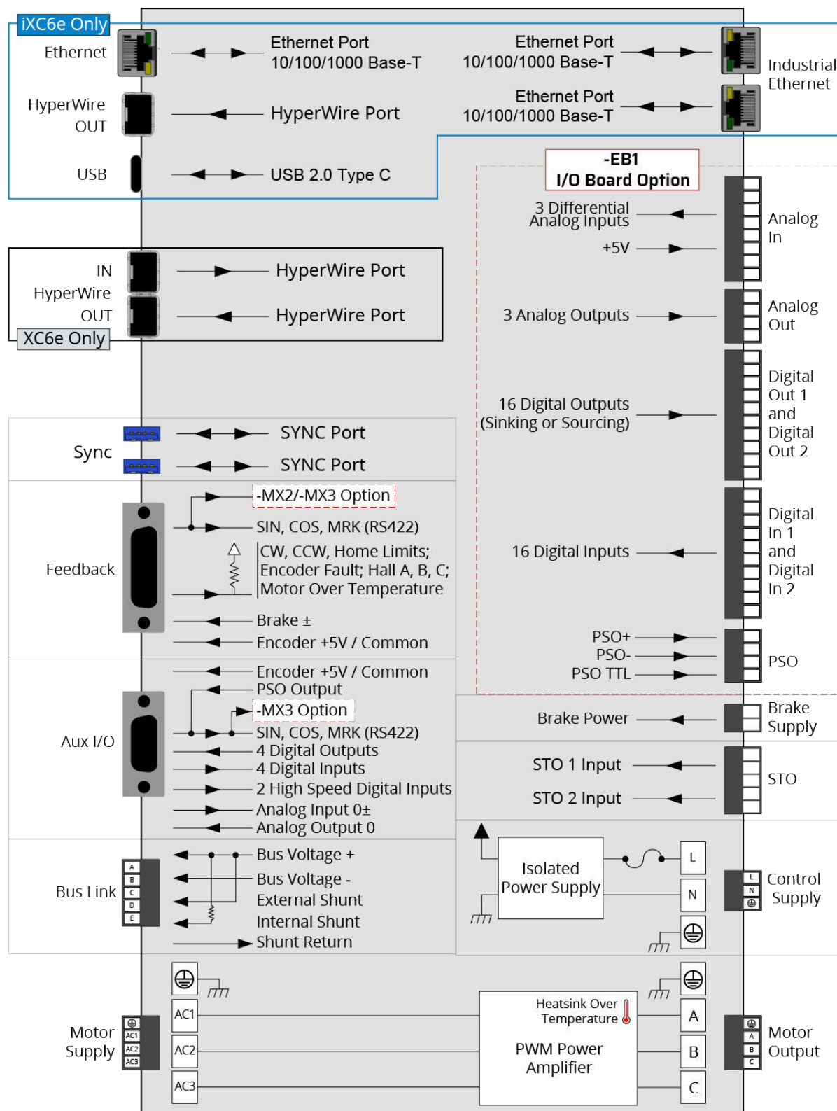
Figure 1-3: Functional Diagram
