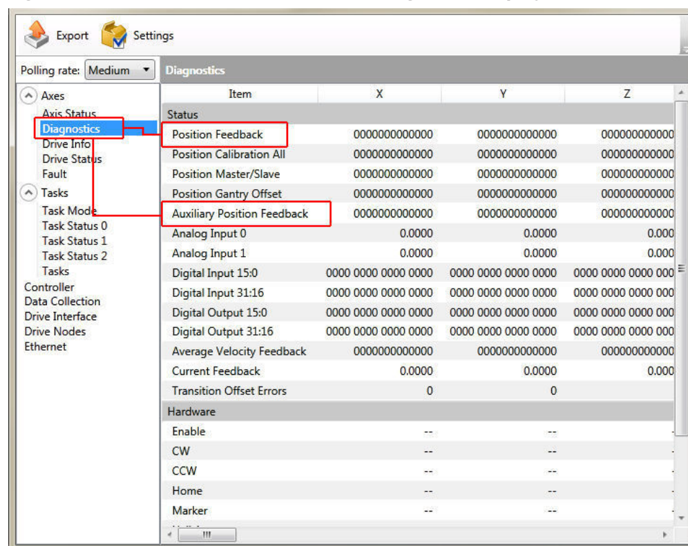
Figure 2-14: Position Feedback in the Diagnostic Display
