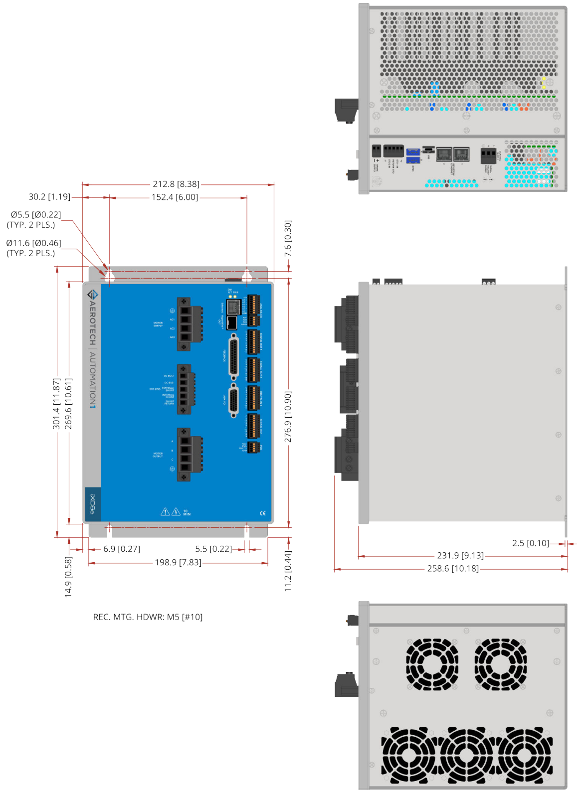
Figure 1-5: Dimensions [-EB1]
