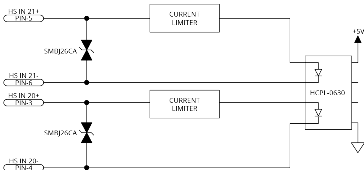
Figure 2-35: High-Speed Inputs
