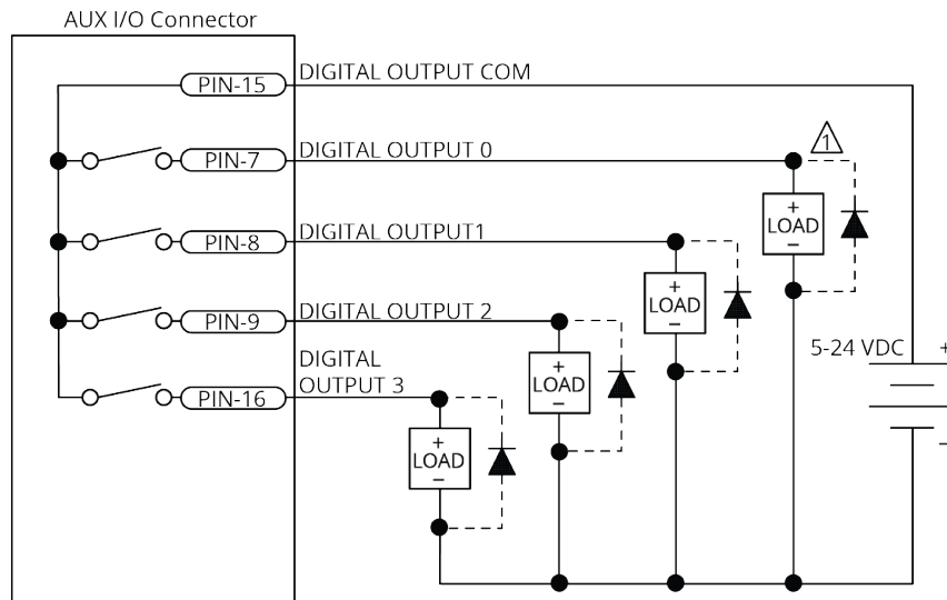
Figure 2-30: Digital Outputs Connected in Current Sourcing Mode
