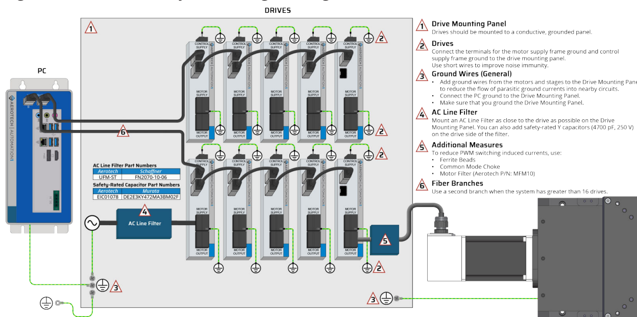
Figure 2-39: PC-Based System Wiring Drawing (Best Practice)
