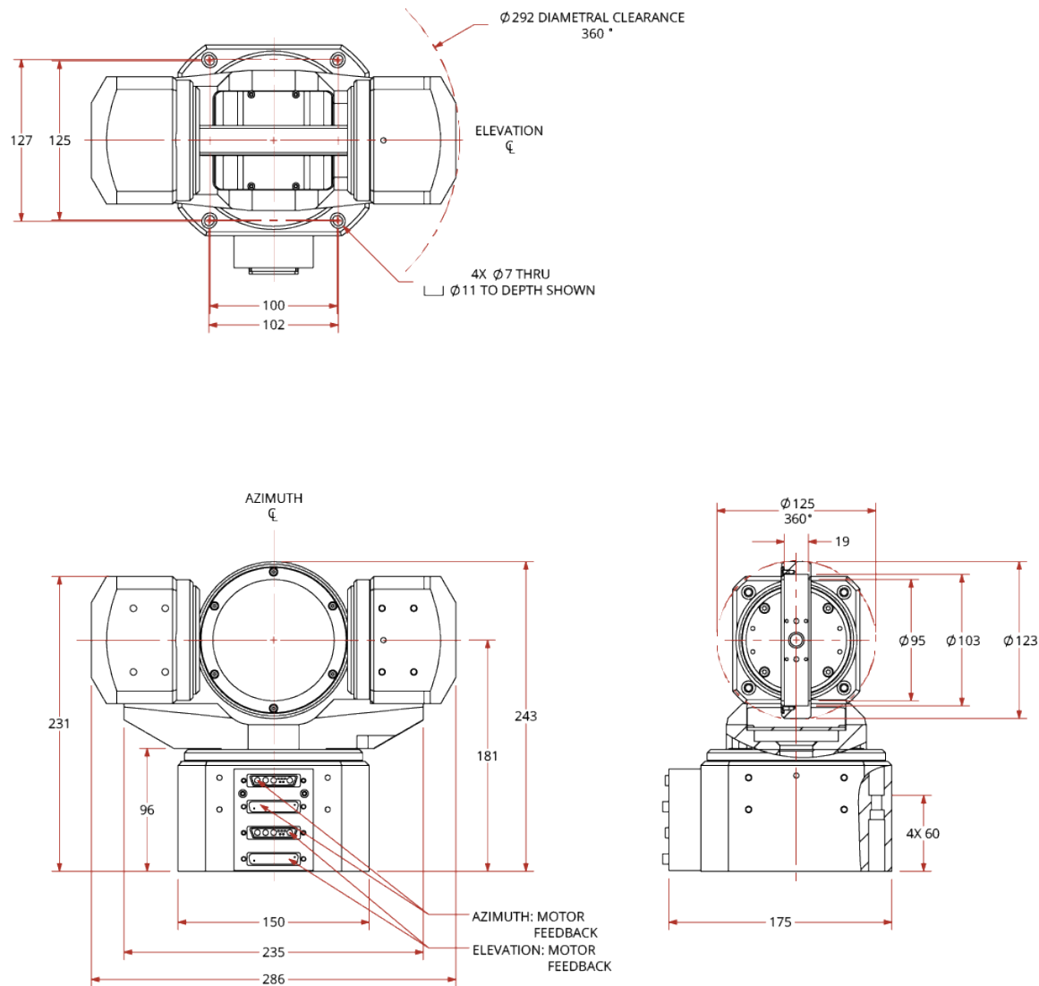
Figure 2-1: AMG100LP Dimensions
