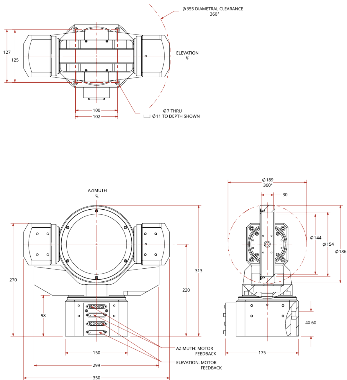
Figure 2-2: AMG150LP Dimensions
