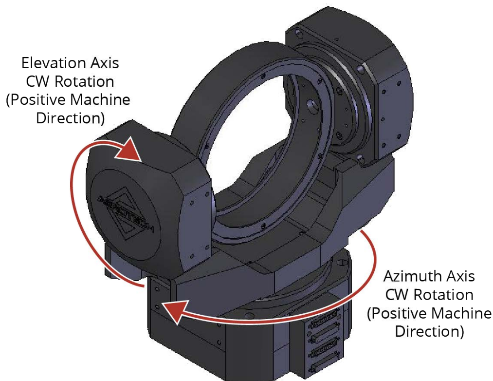
Figure 3-2: Machine Direction
