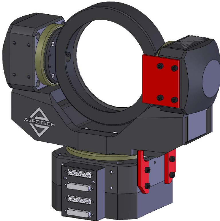
Figure 1-1: Shipping Brackets
