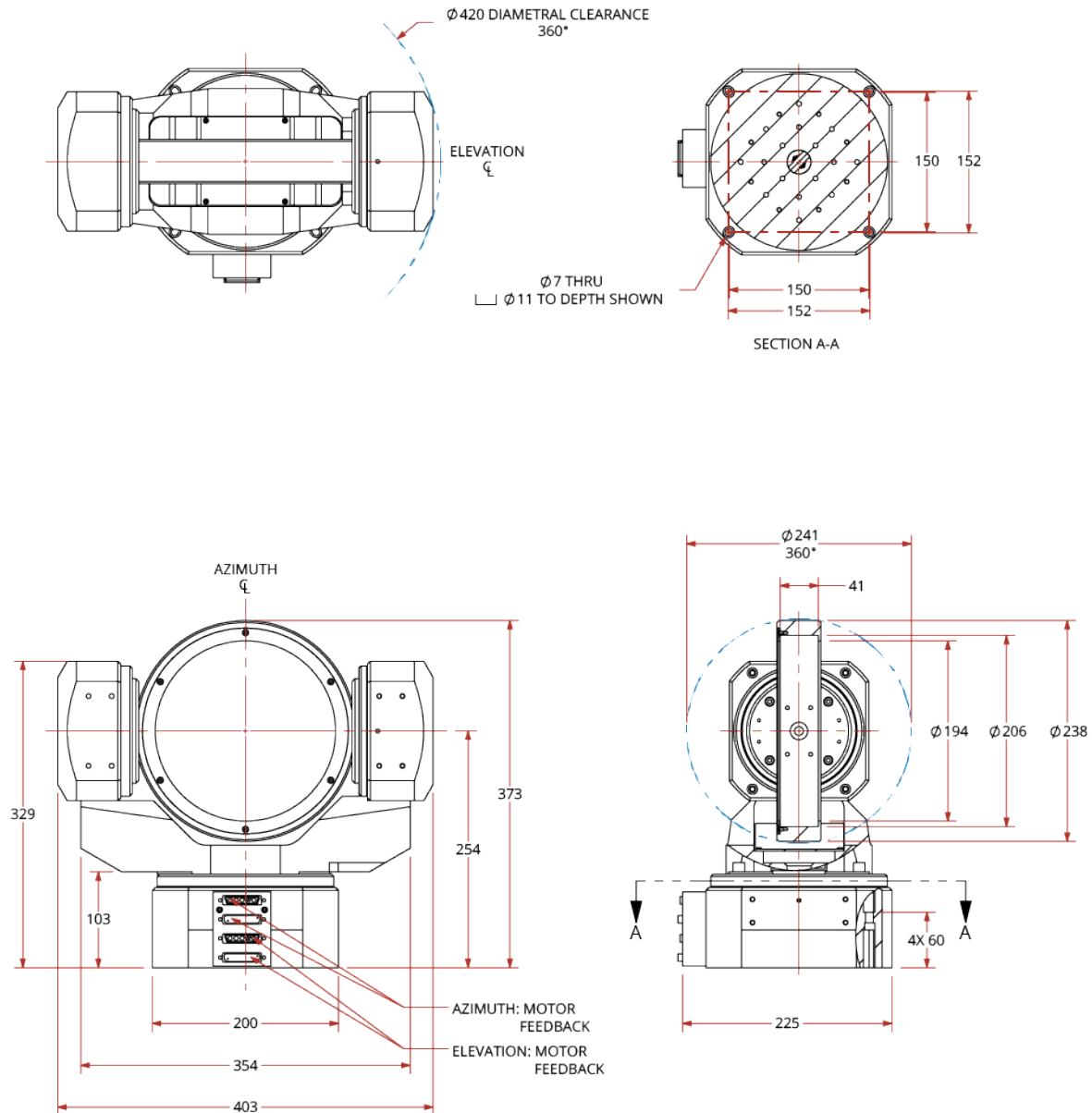
Figure 2-3: AMG200LP Dimensions
