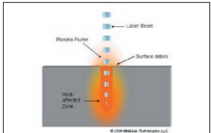
FIG. 7 : SCHEMATIC OF NANO-PULSED LASER PROCESSING
