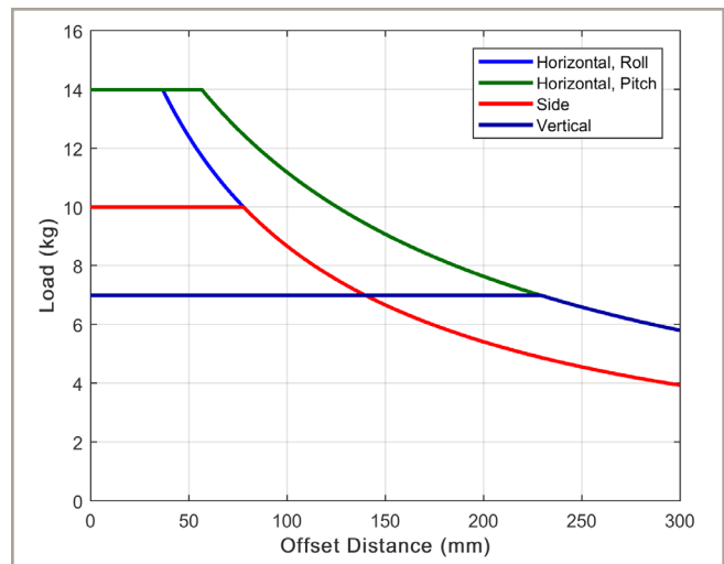
Cantilevered load capability of ATX115SL(E)-100.
