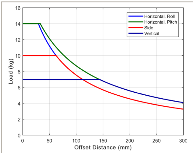
Cantilevered load capability of ATX115SL(E)-050.
