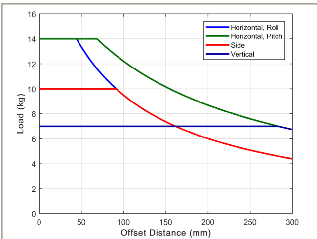
Cantilevered load capability of ATX115SL(E)-150.
