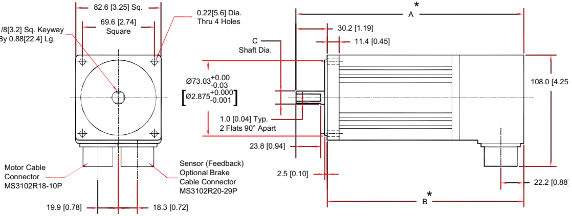
Dimensions - millimeters [inches]
